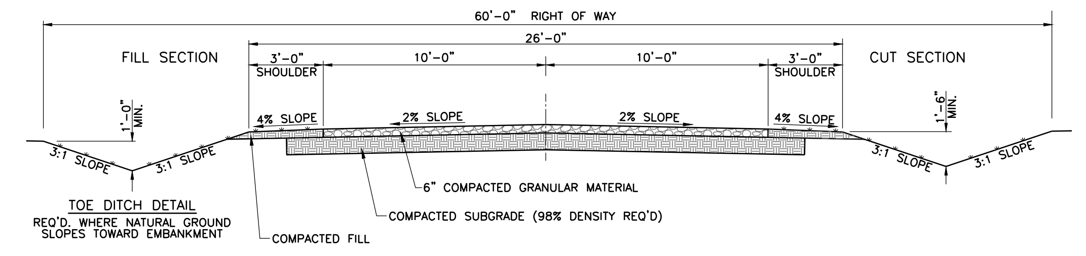
TYPICAL STREET SECTION
